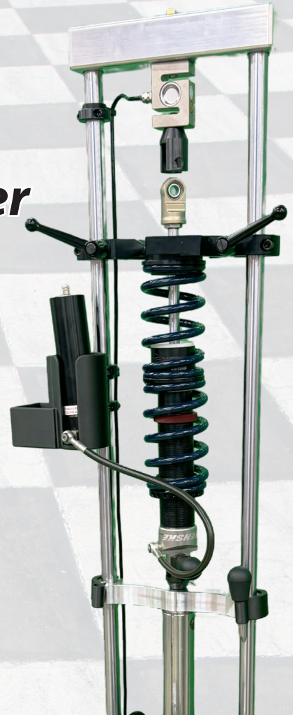
Quick Tap to Zero Load and Travel. Select Push or Pull Mode. (Push Mode Prevents over Extending Shock)
